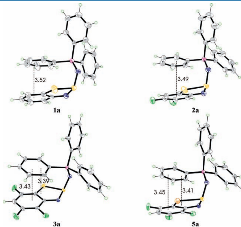
Figure 1. XRD structures of iminophosphoranes 1a–3a and 5a . Color code: gray, C; light gray, H; green, F; blue, N; brown, P; yellow, S; pink, Se (for 2a characterized as 2a \cdot 0.5C_6H_6 , omitted benzene molecules fill lattice cavities and do not interact with the product). For selected bond distances and angles, see Table 3.
